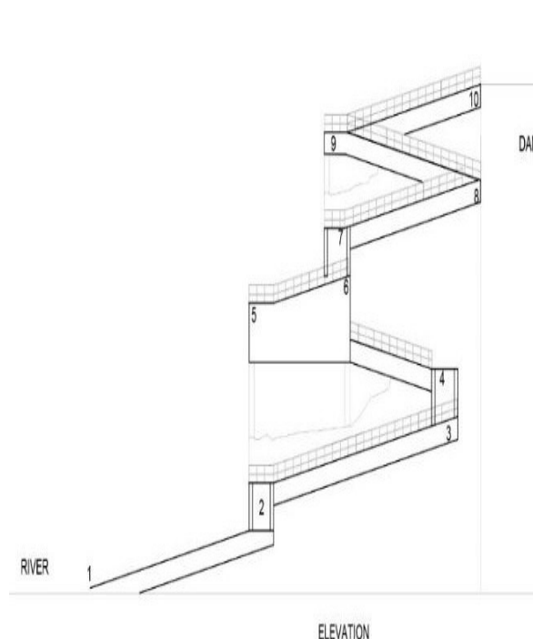
Figure 2. Diagrammatic representation of fishway and sampling sites (4-10).
